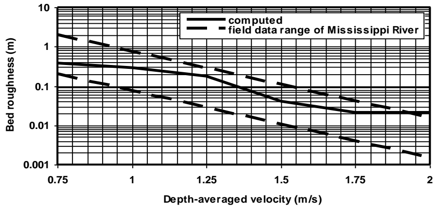
Figure 4 Bed roughness as function of depth-averaged velocity for Mississippi River ( h=10\text{ m} , d_{50}=250\ \mu\text{m} )
