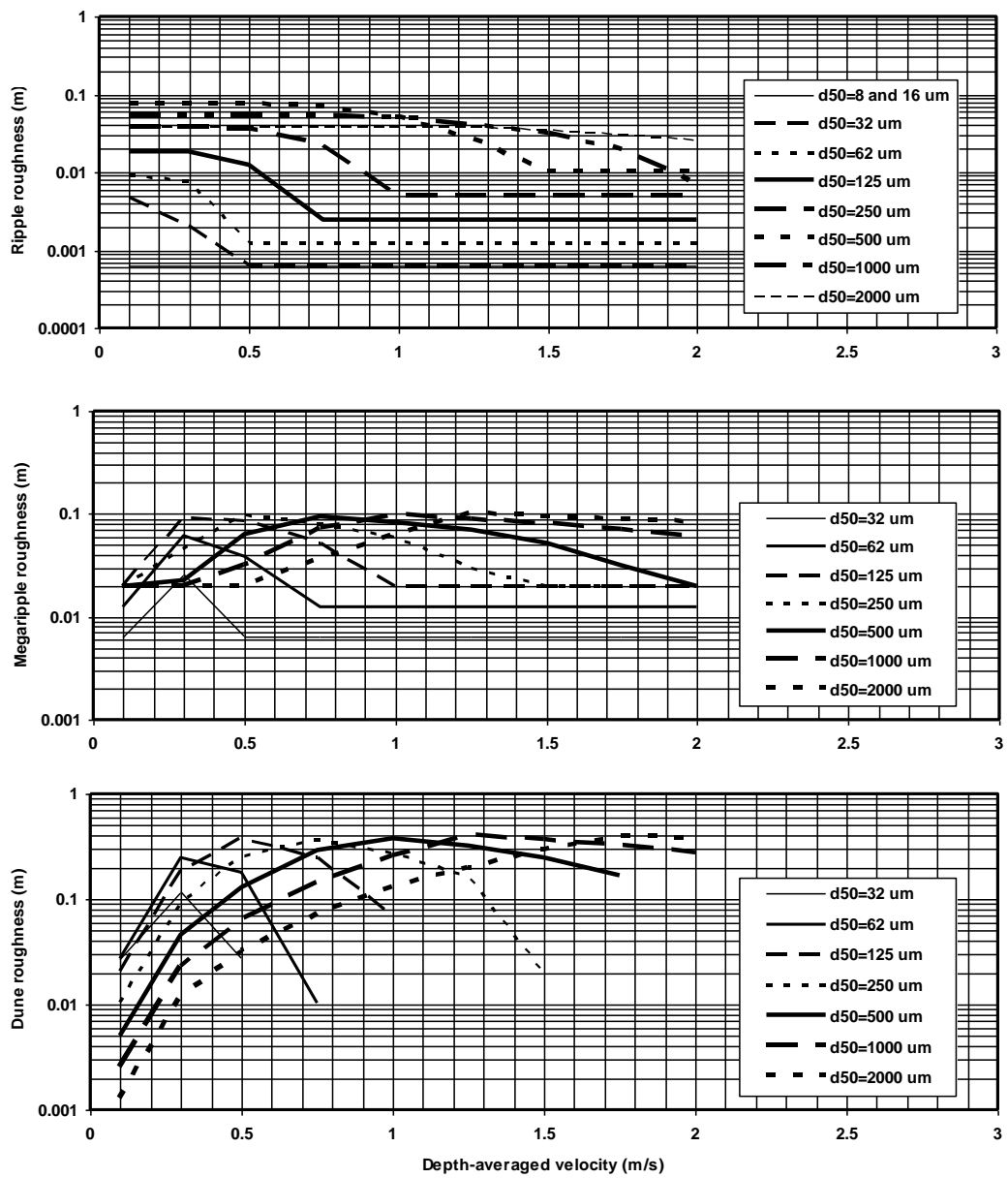
Figure 3 Current-related roughness of ripples (top), megaripples (middle) and dunes (bottom) as function of depth-averaged velocity for sediment of 8 to 2000 \mu\text{m} ( h=10 m)
