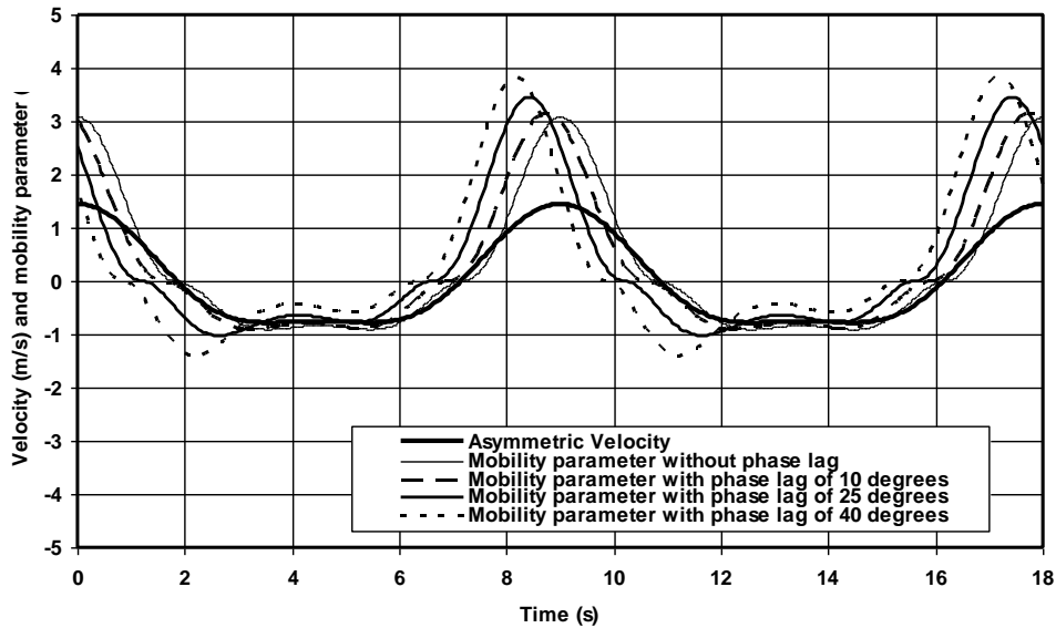
Figure 5 Velocity and Shields mobility parameter ( \theta ) as function of time; asymmetric velocity signal ( U_{max}=1.45 m/s, U_{min}=-0.7 m/s, T=9 s, d_{50}=0.21 mm)
