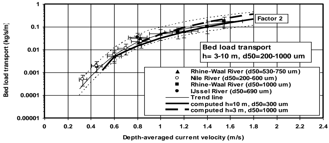
Figure 6 Bed-load transport as a function of current velocity for sand of 200 to 1000 μm
