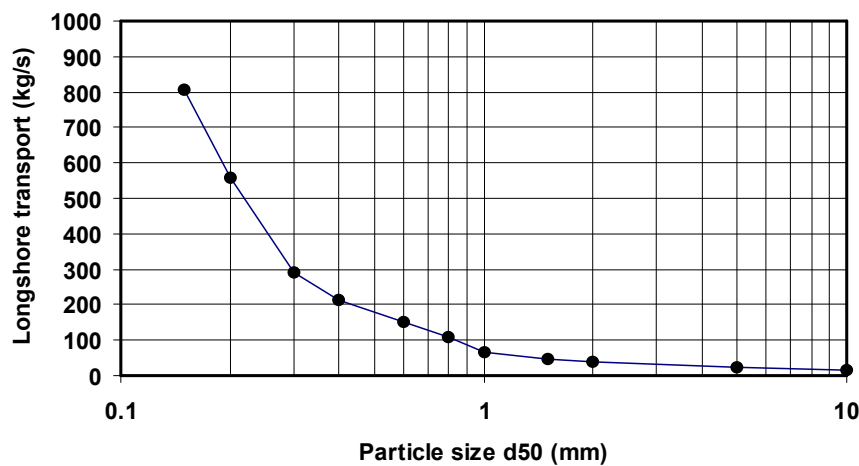
Figure 4 Effect of particle size on longshore transport, offshore wave angle=30°, offshore wave height= 3 m at depth of 15 m
